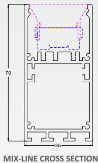
MIX-LINE CROSS SECTION
