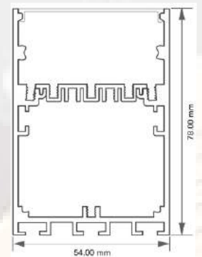
LUMI-LINE CROSS SECTION VIEW
