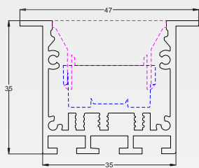
BEAM-LINE CROSS SECTION
